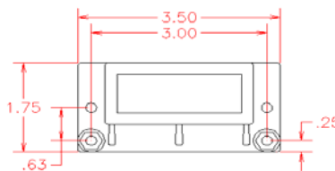
Chassis Mounted CTR-1001
